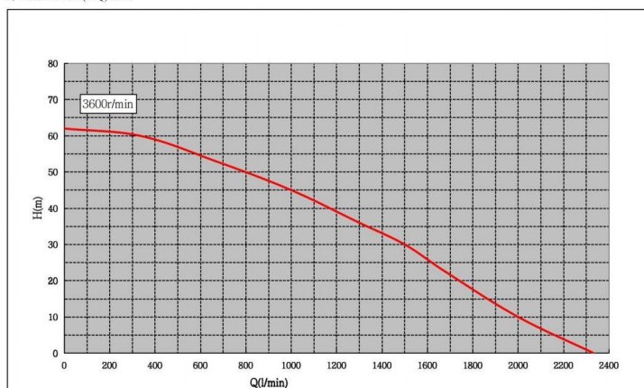
2. Head lift-flow (H-Q) curve
